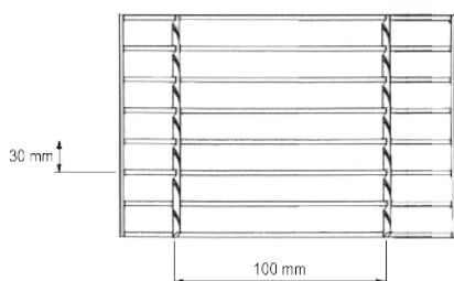
FB 30/100mm Pitch (Plain)
