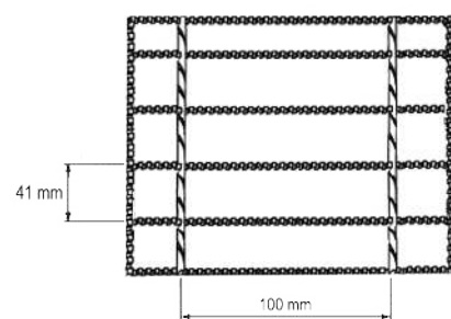
FB 41/100mm Pitch (Serrated)
