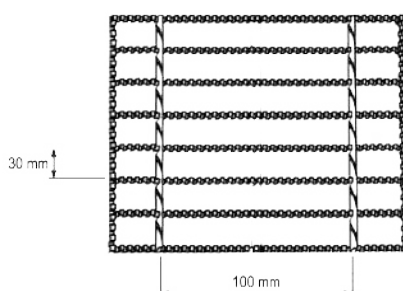
FB 30/100mm Pitch (Serrated)
