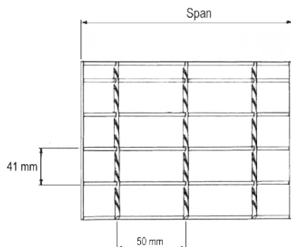
FB 41/50mm Pitch (Plain)
