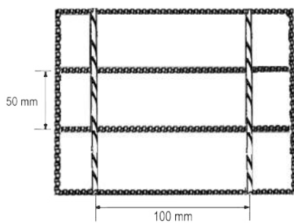
FB 50/100mm Pitch (Serrated)
