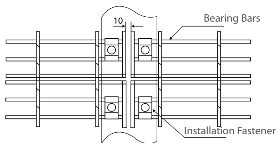
Diagram for Fastener Installation
