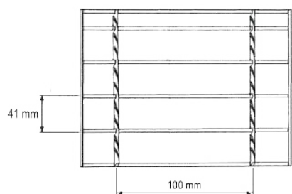
FB 41/50mm Pitch (Serrated)
